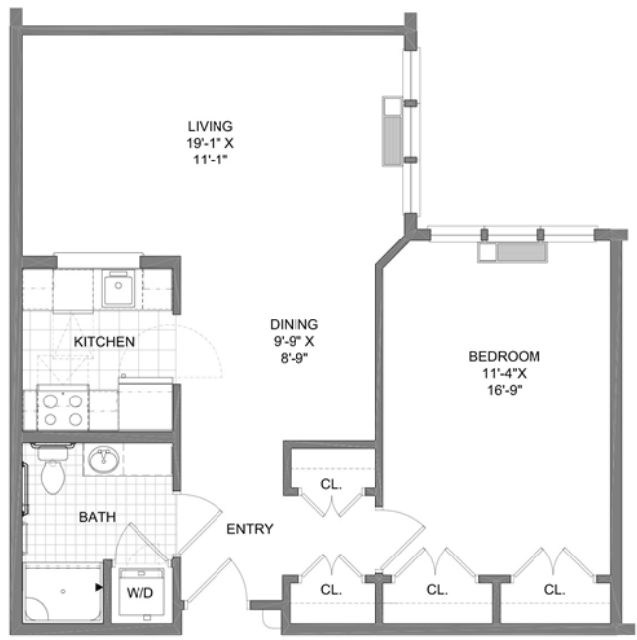
UNIT TYPE ABL-1Bd- OPTION 1 792 SQ. FT.
